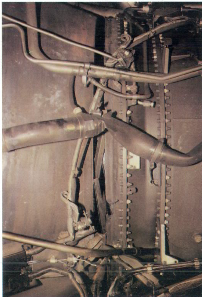
PHOTOGRAPH SHOWING CIRCUMFERENTIAL FRACTURE OF TURBINE CASE
