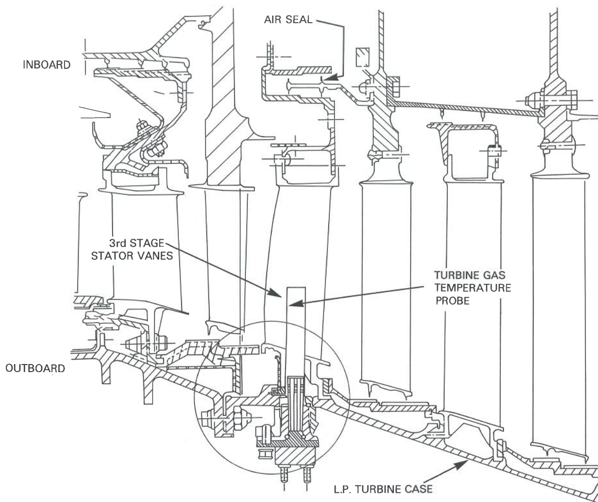
SECTION OF ENGINE SHOWING LOW PRESSURE STATOR VANE LOCATION
