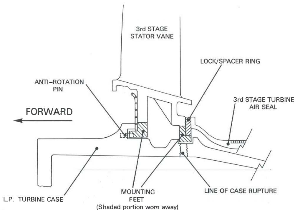
EXPANDED VIEW OF STATOR LOCATION ( T.G.T. PROBE OMITTED FOR CLARITY )
