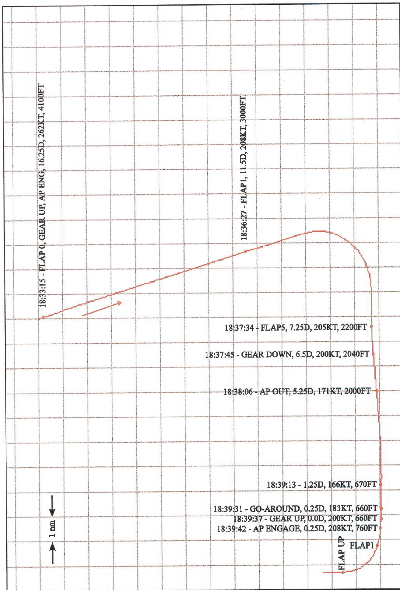
First missed approach (ground track)
