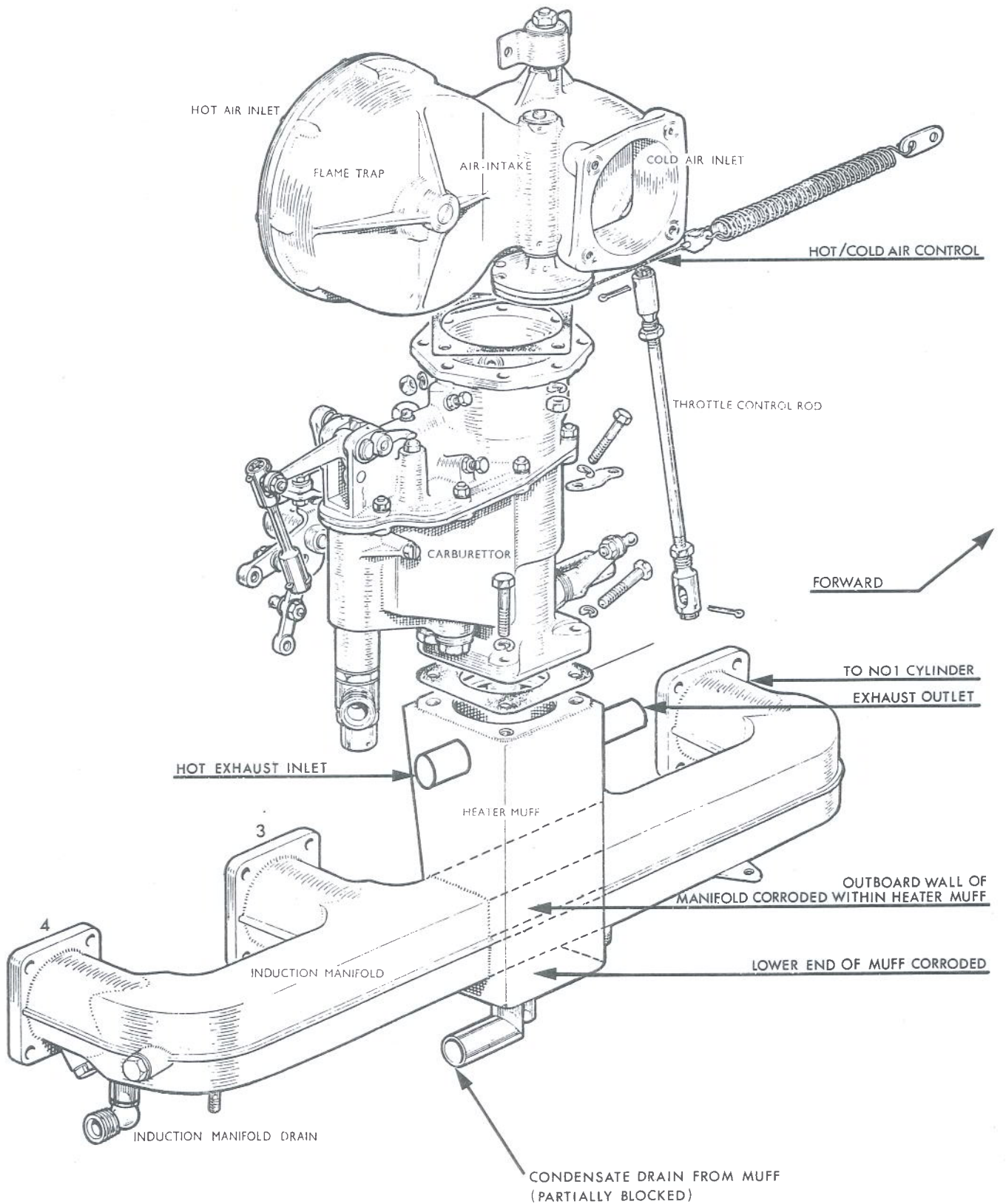
AIR INTAKE, CARBURETTOR, AND MILD STEEL INDUCTION MANIFOLD ASSEMBLY AS FITTED TO THE GIPSY MAJOR ENGINE ON THE BEAGLE TERRIER G-ARZT
